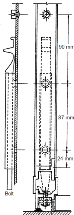
Fig. 21.26 : Typical Vertical Bolt for Double Shutter Door
