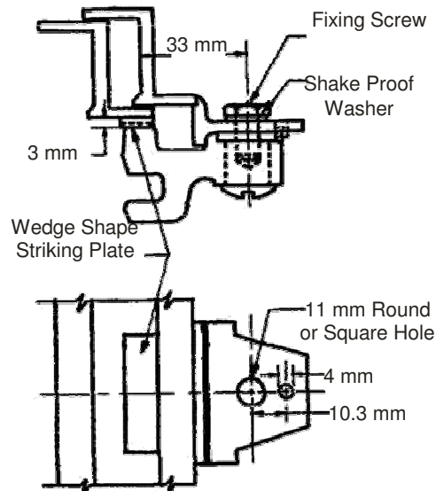
Fig. 21.15 : A Typical Handle for Side-Hung Shutter
