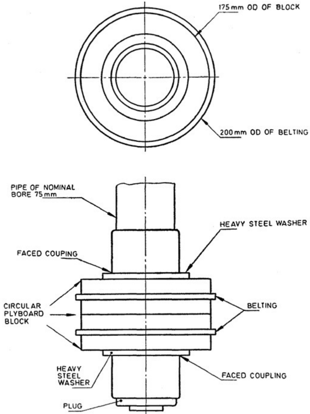
Fig. 23.13 Surge Block
