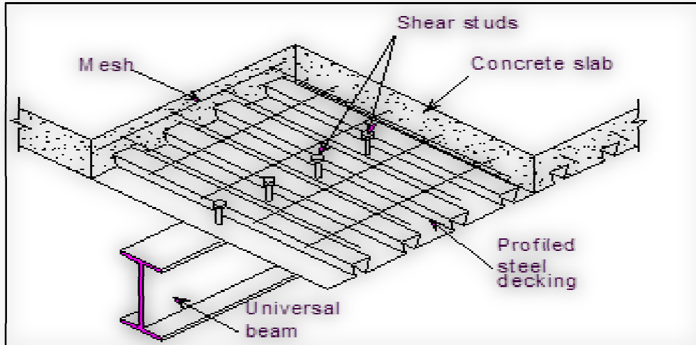
Fig 26.14 Galvanized Steel Deck Sheet
