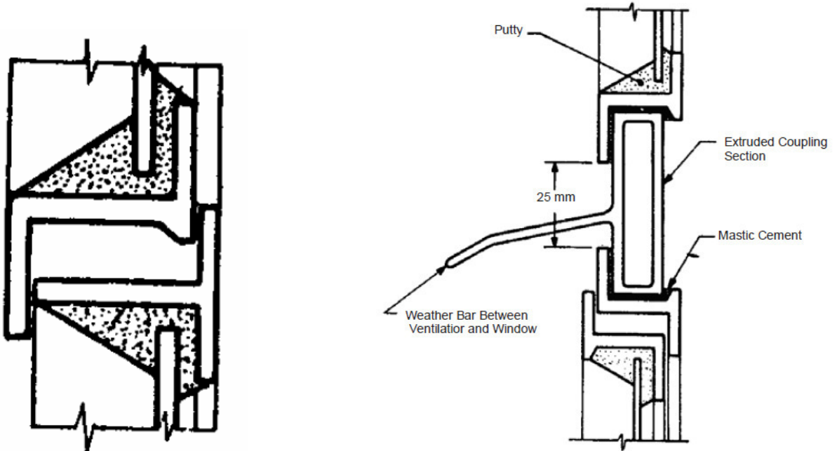
Fig 21.7 : Coupling Section Extruded for Coupling Windows Side by Side
