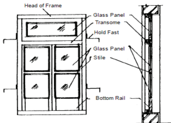
GLAZED AND PANELLED DOOR
