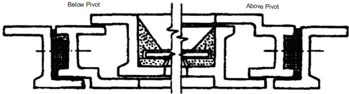
Fig. 21.20 : Detail of Horizontal Centre-Hung Ventilator
