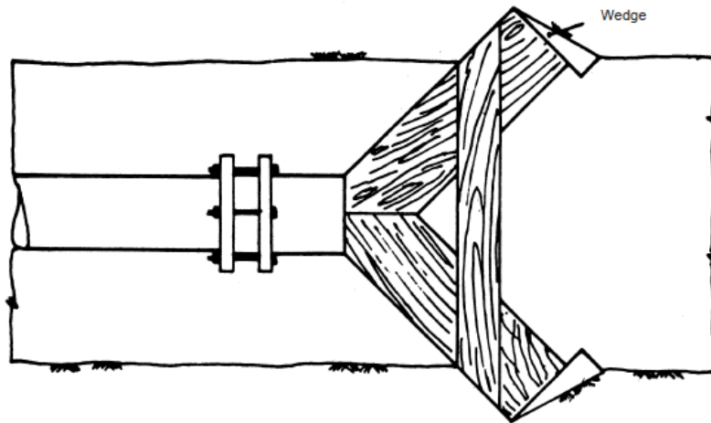
FOR PIPES UPTO 125 NOMINAL DIA
