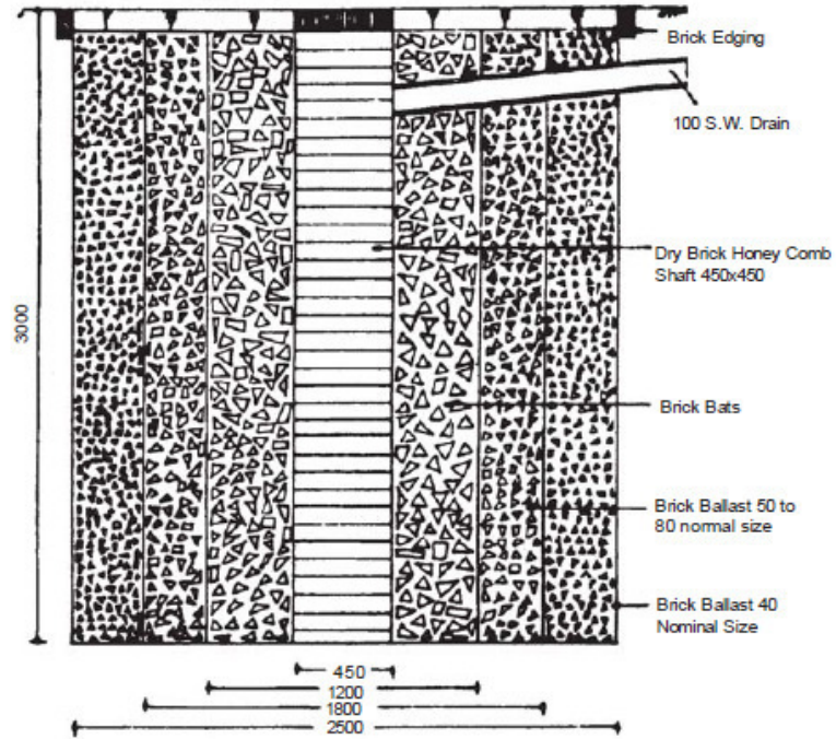
SECTION AB
