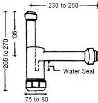
TYPICAL DETAIL OF BOTTLE TRAP
