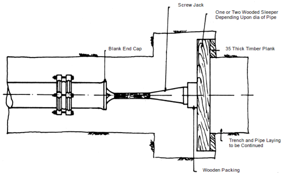
FOR PIPES OF NOMINAL DIA OVER 125
