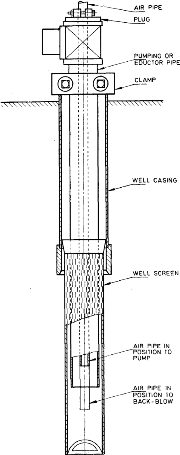
FIG. 23.12 Open Well Development with Air Compressor
