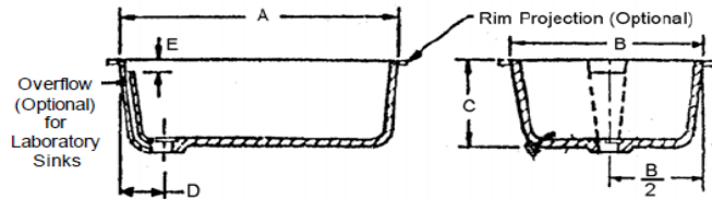
KITCHEN AND LABORATORY SINKS (WHITE GLAZED FIRE CLAY)
