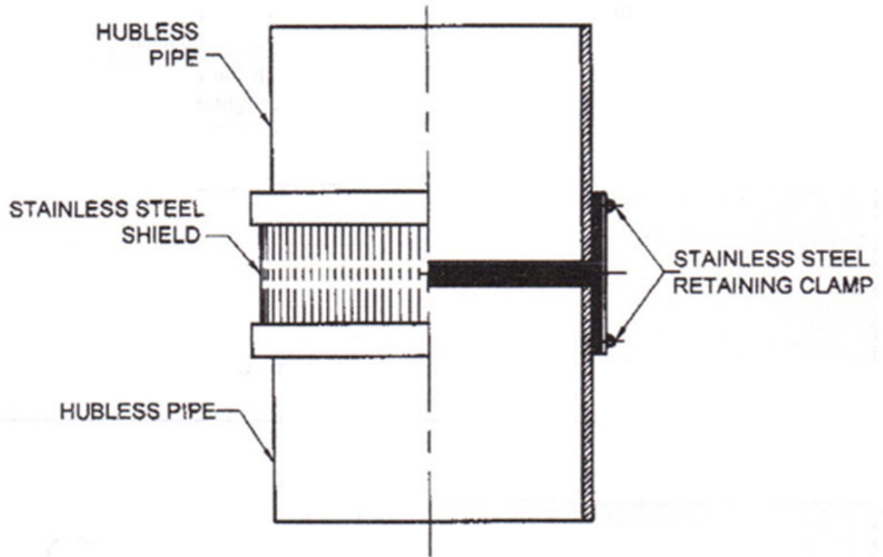
Fig. 17.24 Typical coupling joint-installation
