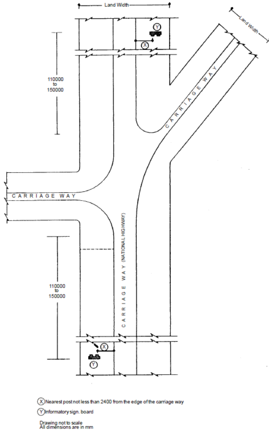
Fig. 16.11 : Location of Informatory Sign Boards
